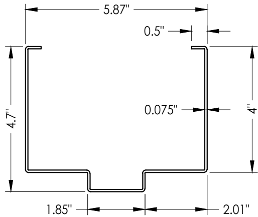
26 FRAME
