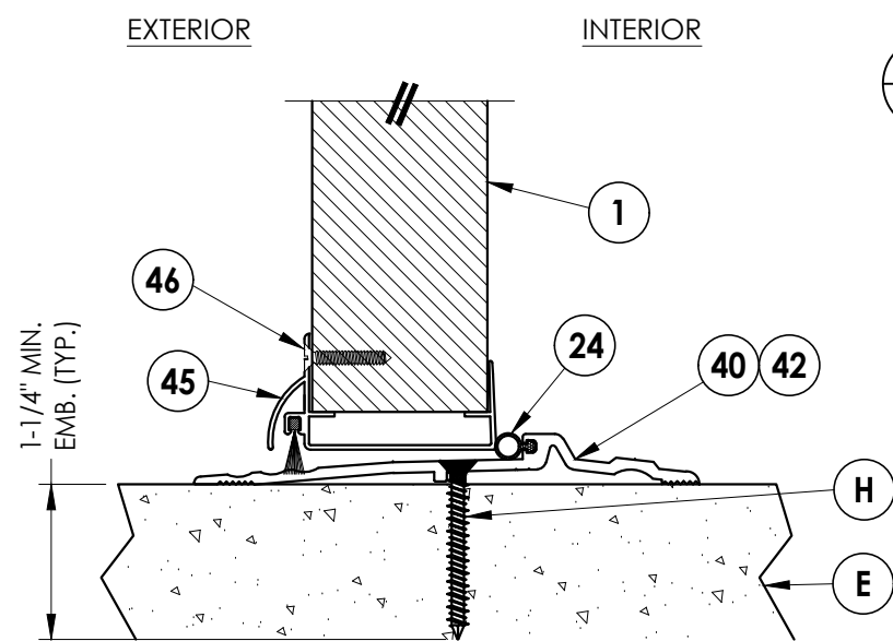
4 VERTICAL CROSS SECTION
