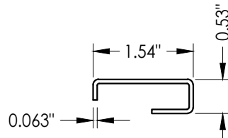
86A GLASS STOP
