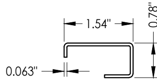
86 GLASS STOP
