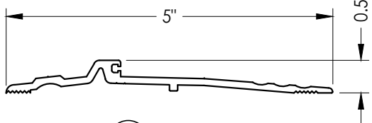
40 THRESHOLD
