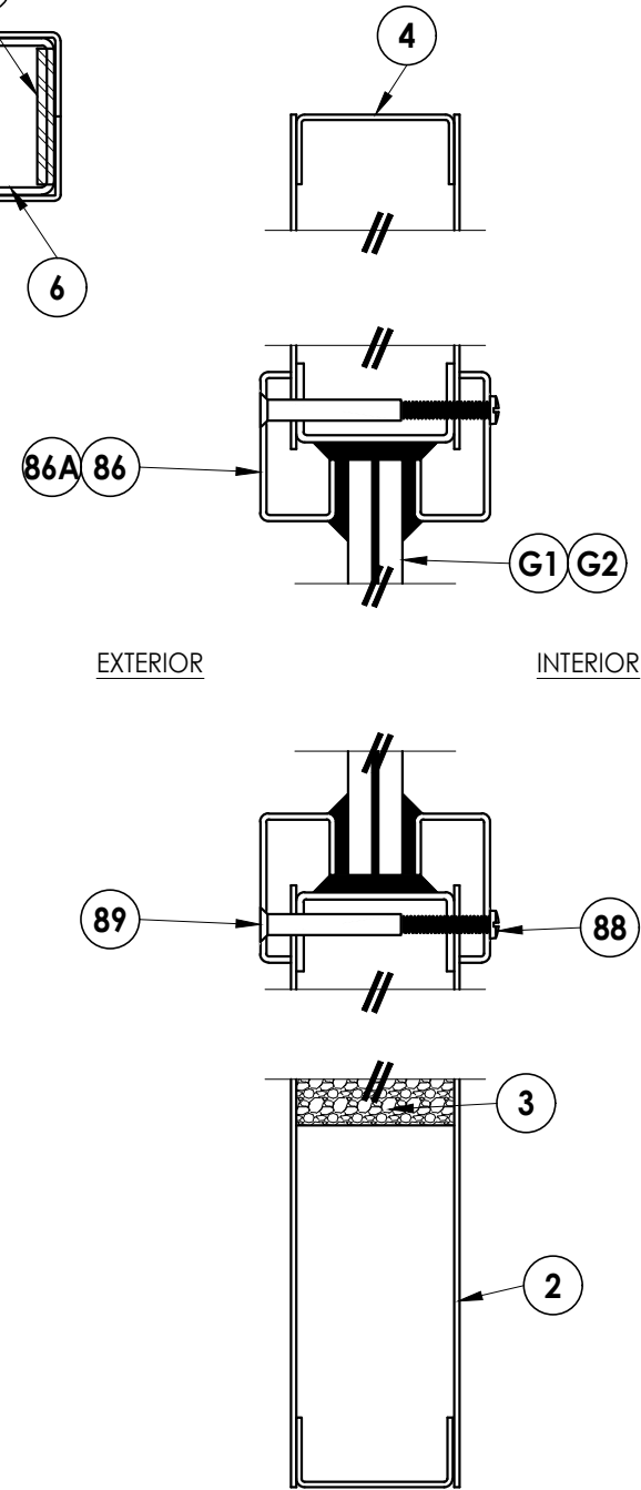
VERTICAL CROSS SECTION
