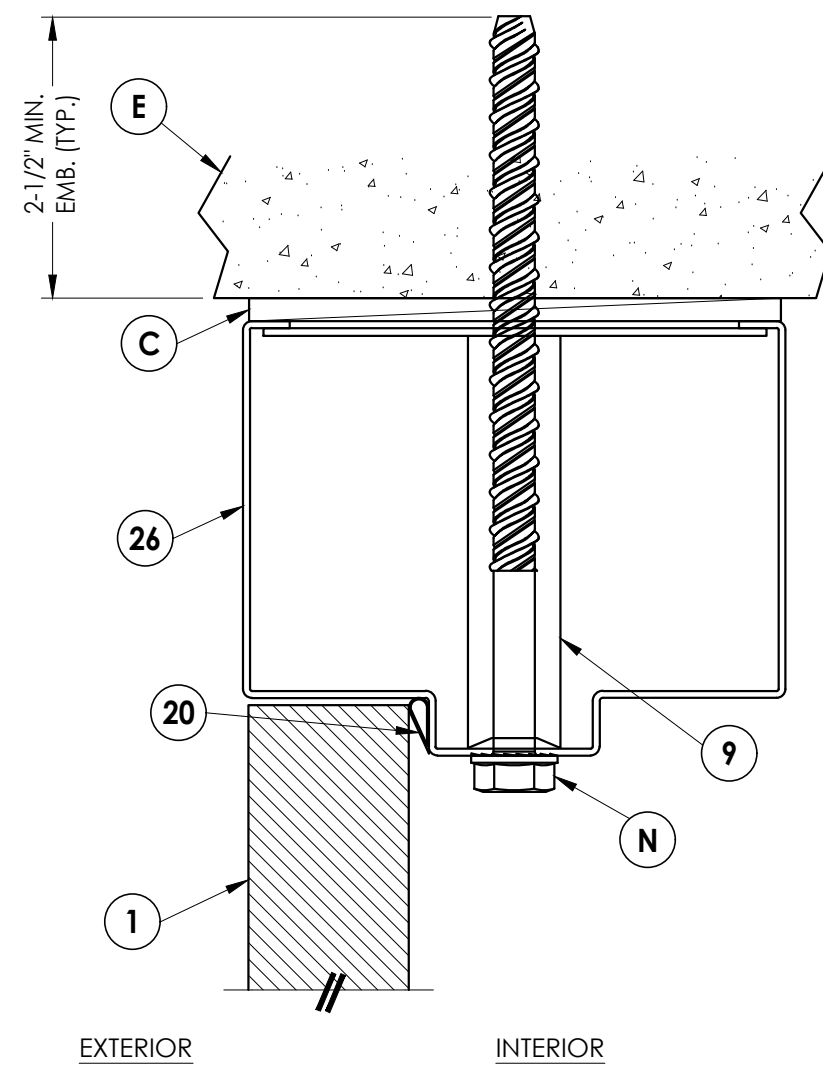
2 VERTICAL CROSS SECTION 4
