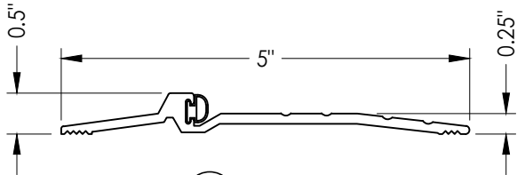
42 THRESHOLD
